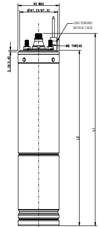
FIGURE 1: 2-WIRE MOTOR
